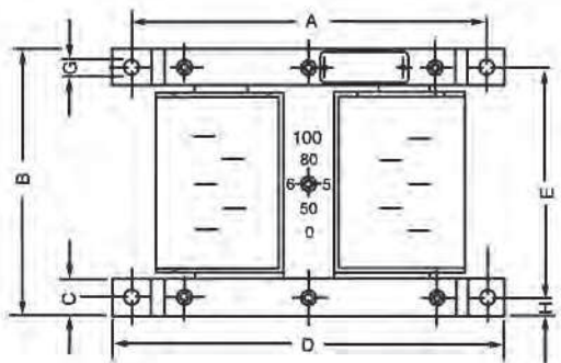
Vista Frontal
